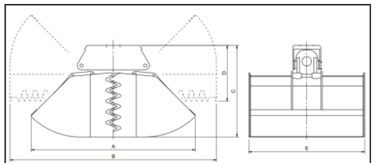
HEMA Flisgrab FG90-3000
